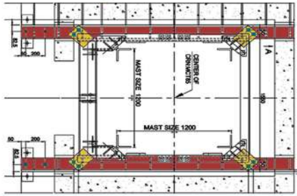
Climbing Collar Plan
